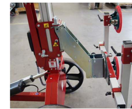
The extension diagonally downwards enables narrow discs to be accommodated
